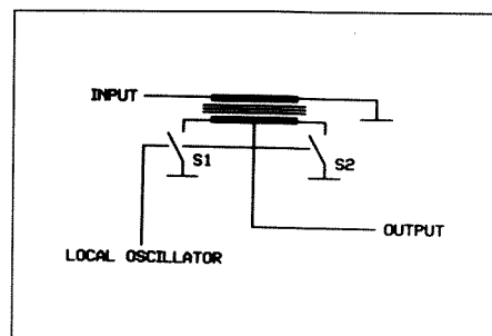
Figure 2. Illustration of mixer action used in the filter.
