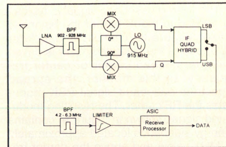
Figure 12. Image rejection receiver block diagram.
