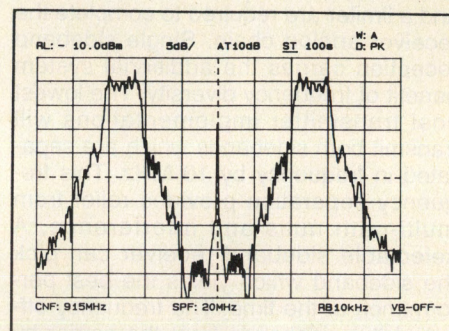
Figure 9. Typical modulated DSB spectrum.
