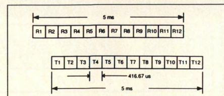
Figure 1 - TDD/TDMA frame structure for DECT.
