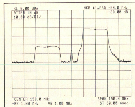
Figure 3. IF output of SSB modulator.
