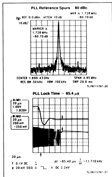
Figure 4 - Lock time and spurious noise performance of National's PLL for the DECT transceiver.
