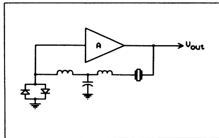
Figure 6. The oscillator with a complete feedback circuit.
