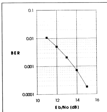
Figure 6 - Simulated BER for the DECT receiver.
