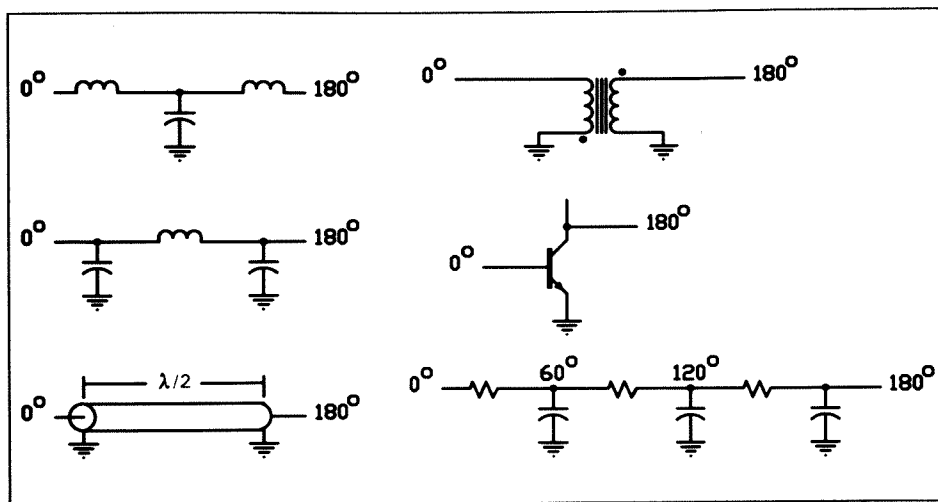
Figure 4. Methods of obtaining the necessary 180-degree phase shift.
