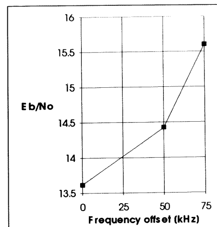
Figure 7 - Required E_b/N_o as a function of the frequency offset on the received signal.
