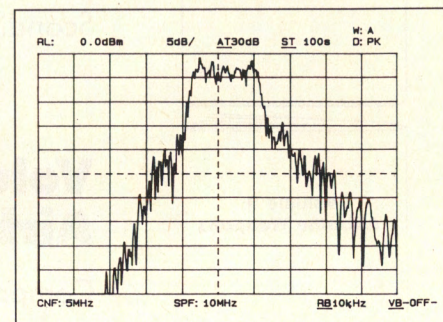
Figure 7. Baseband transmit spectrum after filtering.
