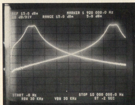
Figure 4. Filter response at either end of its tuning range.
