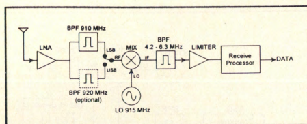
Figure 10. Single conversion receiver block diagram.
