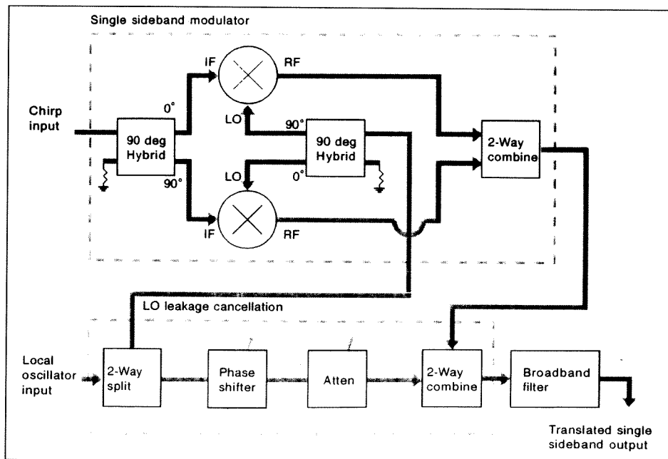
Figure 2. Block diagram of SSB upconverter including single sideband modulator, LO cancellation circuit, and broadband filtering.
