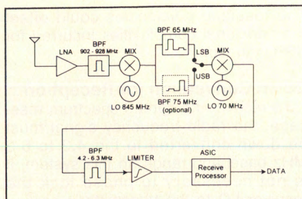
Figure 11. Double conversion receiver block diagram.
