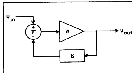
Figure 1. The classic representation of negative feedback.
