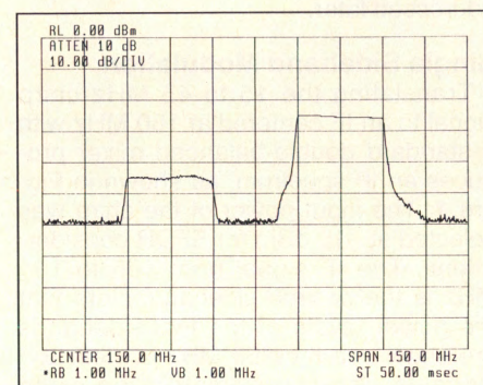
Figure 4. IF output of SSB modulator with LO cancellation.
