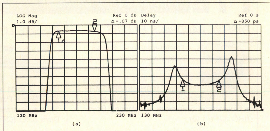
Figure 5. Bandpass filter response a) log magnitude and b) group delay.
