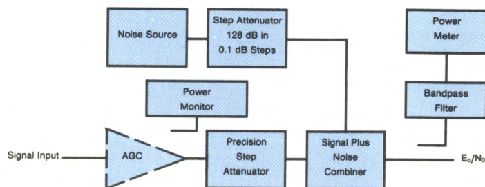
Figure 1. Block Diagram of UFX-BER Series Instrument.
