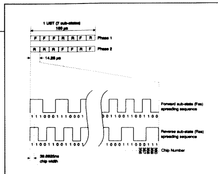
Figure 3. UST and sub-state timing.
