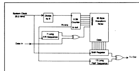
Figure 5. Transmit processor.
