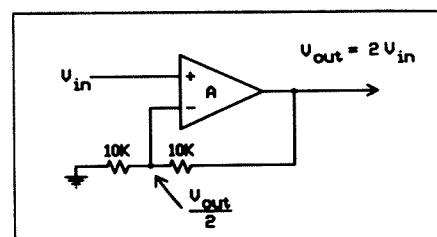
Figure 2. A simple gain-of-2 operational amplifier example.
