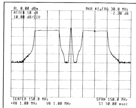
Figure 1. IF output of standard double balanced mixer.
