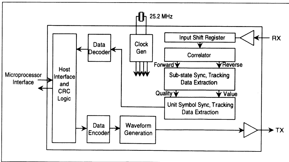
Figure 1. Block diagram of modem ASIC.
