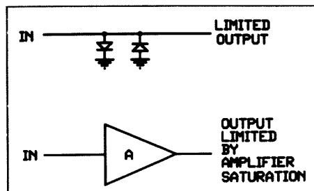
Figure 5. Two ways to limit amplitude.
