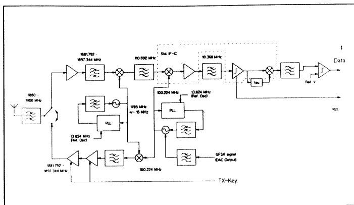
Figure 2 - A block diagram of a typical 2 GHz radio.
