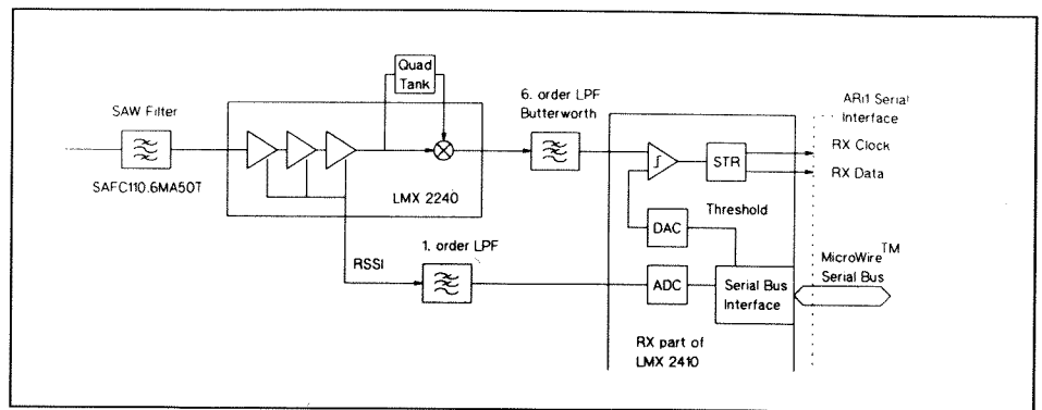
Figure 5 - Simplified block schematic for a DECT transceiver.
