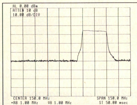
Figure 6. IF output of SSB modulator with LO cancellation and filter.
