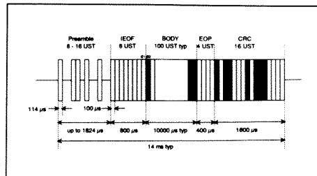
Figure 2. Typical packet timing.
