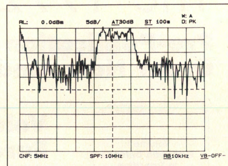
Figure 6. Baseband transmit spectrum before filtering.
