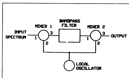
Figure 1. Block diagram of swept filter
